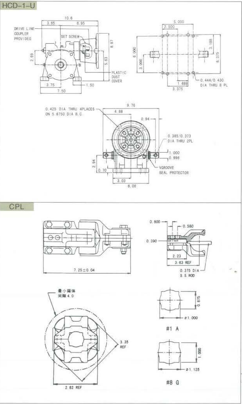
安装图 Dimensional Drawing
