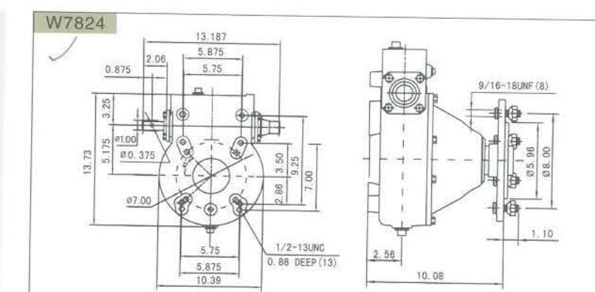
安装图 Dimensional Drawing
