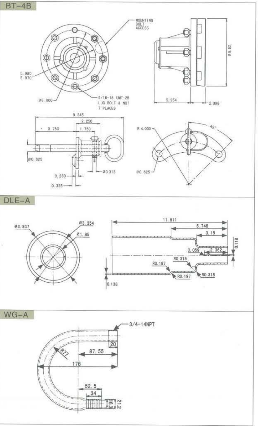
安装图 Dimensional Drawing
