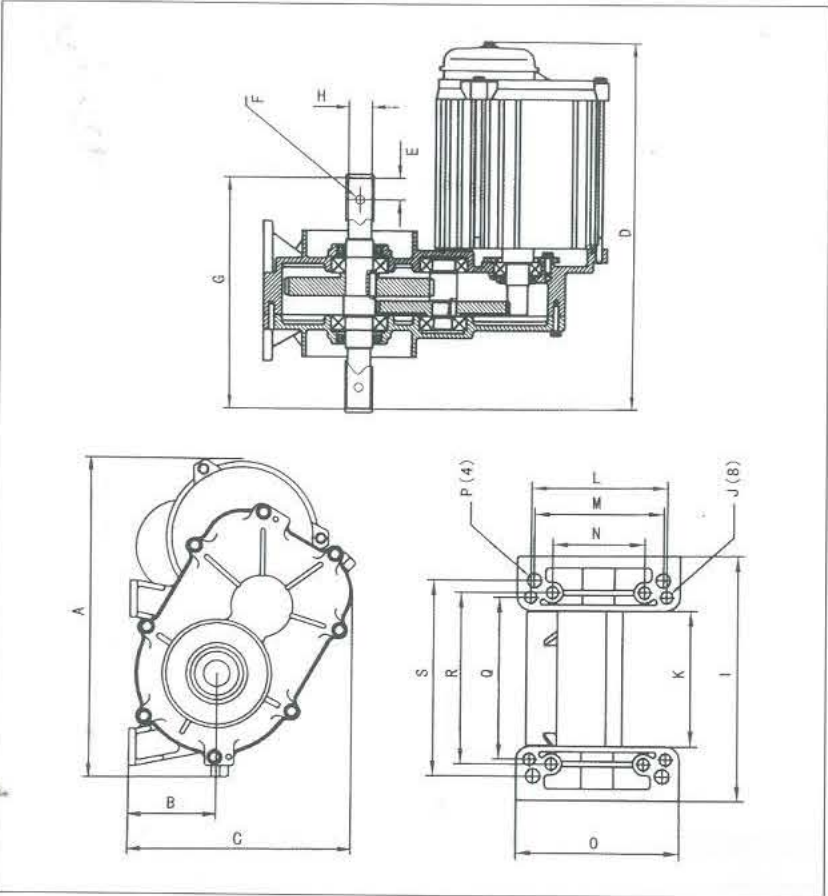
安装图 Dimensional Drawing
