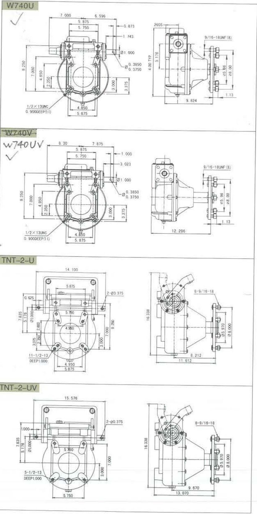
安装图 Dimensional Drawing
